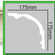
C 756 175x175mm L:2440mm
