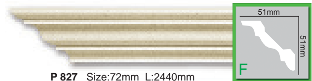
P 827 Size:72mm L:2440mm
