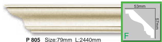
P 805 Size:79mm L:2440mm
