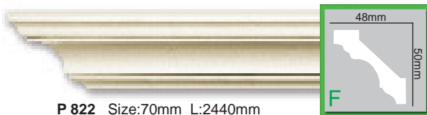
P 822 Size:70mm L:2440mm
